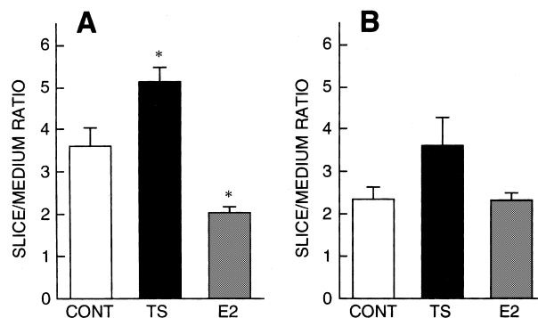
Fig. 3. TEA accumulation by kidney slices from male and female rats treated with testosterone and estradiol. Kidney slices from males (A) and females (B) were incubated at 25°C in buffer containing 50 \mu M [ ^{14} C]TEA for 60 min. CONT, rats treated with vehicle; TS, rats treated with testosterone; E2, rats treated with 17 \beta -estradiol. Each column represents the mean \pm S.E.M. of three separate experiments in three slices. * P < 0.05, significantly different from control.
